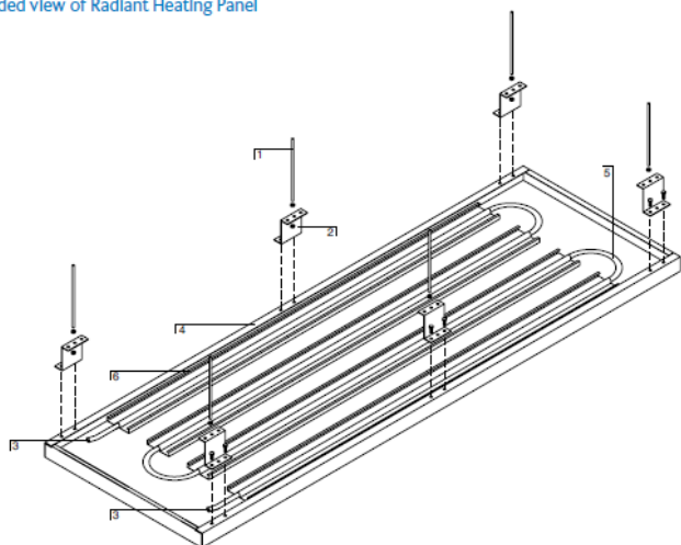
Exploded view of Radiant Heating Panel
